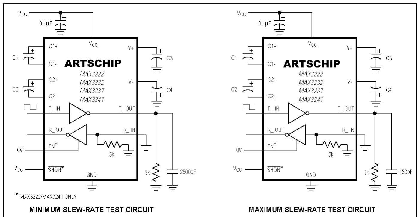
Figure 1. Slew-Rate Test Circuits
