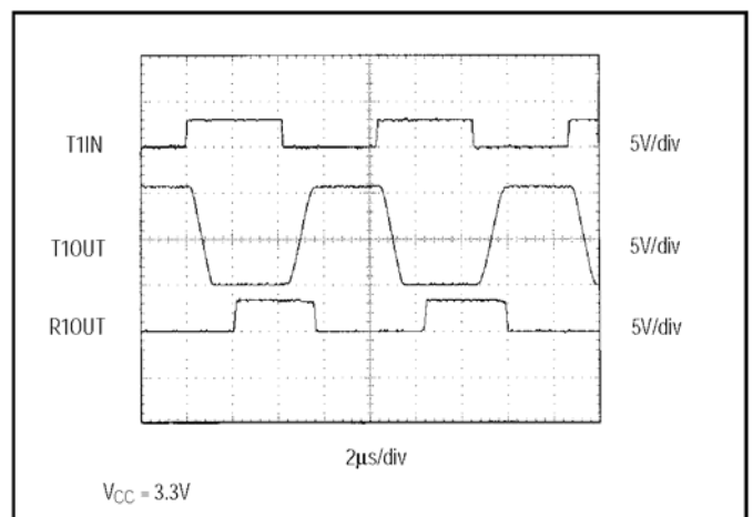
Figure 7. MAX3241 Loopback Test Result at 235kbps
